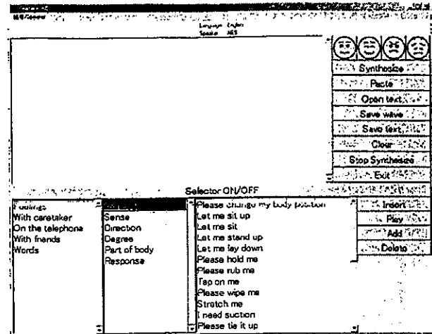
Figure 3: List window
