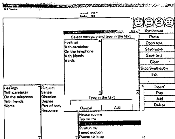
Figure 4: Add window.
